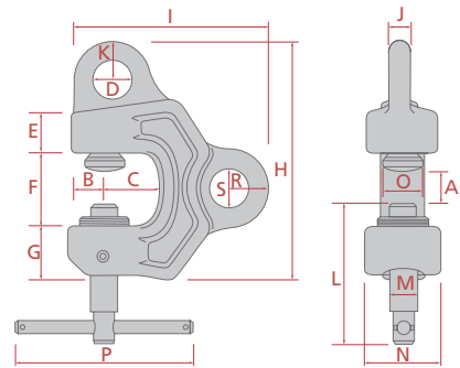
Measurement diagram for SSB and SSBA
