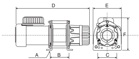
Single Phase Model
